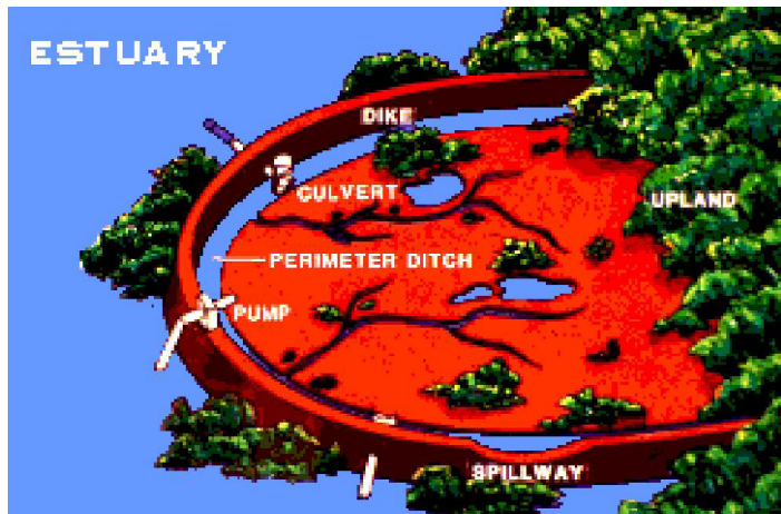
Figure 1. Impoundment schematic.
